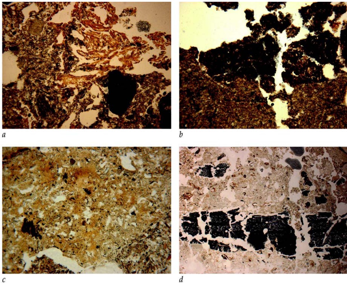
Fig. 16. Test Pit 5 (2012) soil photomicrographs (C. French/D. Redhouse): a . Photomicrograph of micritic ash with abundant fine fragments of uncarbonised and partly humified and silicified plant remains, many phytoliths and recognisable fragments of grass stems and leaves, as well as anthropogenic inclusions of pottery fragments, unfired clay aggregates and degraded bone, sample 10/3 (frame width = 4.5mm; plane polarized light); b . Photomicrograph of the upper surface contact of the compacted micritic ash and silty clay with the humic silty clay above, sample 10/4 (frame width = 4.5mm; plane polarized light); c . Photomicrograph of the considerable quantities of included degraded bone (i.e. amorphous yellow areas) in the upper surface contact, sample 10/4 (frame width = 2.25mm; plane polarized light); d . Photomicrograph of the micritic ash fabric with horizontal organisation of wood charcoal fragments, sample 10/4 (frame width = 2cm; plane polarized light)
