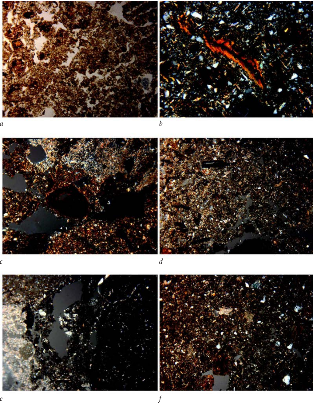
Fig. 15. Test Pits 1 and 4 (2011) soil photomicrographs (C. French/D. Redhouse): a. Photomicrograph of the pellety very fine sandy silty clay fabric, Sample 1/1, Test Pit 1 (frame width = 4.5mm; plane polarized light); b. Photomicrograph of the reticulate striated fabric with a pure to fine dusty crescentic clay infill of a void, Sample 1/1, Test Pit 1 (frame width = 2.5mm; cross polarized light); c. Photomicrograph of the heterogeneous mixture of very fine sandy silty clay loam in pellety to irregular aggregates, wood ash with abundant fine charcoal and irregular aggregates of amorphous iron 'cemented' clay and sparite, Sample 4/1, Test Pit 4 (frame width = 2.5mm; plane polarized light); d. Photomicrograph of the heterogeneous mixed fabric of calcitic ash with fine charcoal fragments and the very fine sandy silty clay loam soil fabric, upper part of Sample 4/2, Test Pit 4 (frame width = 4.5mm; cross polarized light); e. Photomicrograph of partially humified and calcite replacement of plant tissue, Sample 4/2, Test Pit 4 (frame width = 2.5mm; cross polarized light); f. Photomicrograph of the very fine sandy silty clay loam fabric with included micritic ash and fine charcoal, Sample 4/3, Test Pit 4 (frame width = 4.5mm; cross polarized light)
