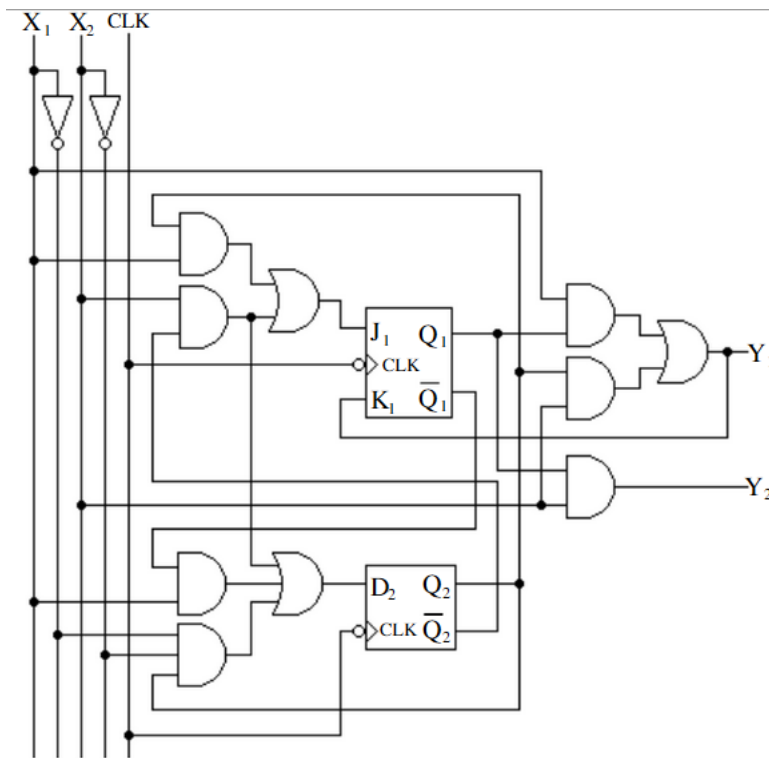
Figure 3. Logical scheme
