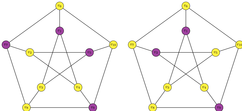
FIGURE 1. A minimal (on the left) and a minimum dominating sets of the Petersen graph.
