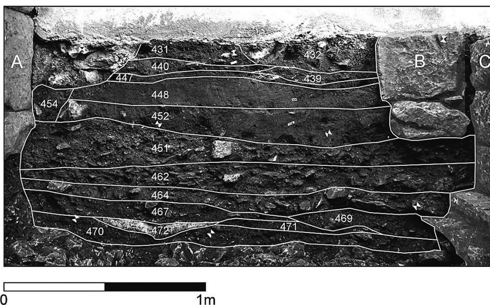
Fig. 14. Western section of trench L13. A = Inner face of the south fortification wall, B = repairs of the water intake construction, C = water intake construction (after Popović / Devlahović 2018, Fig. 17)
