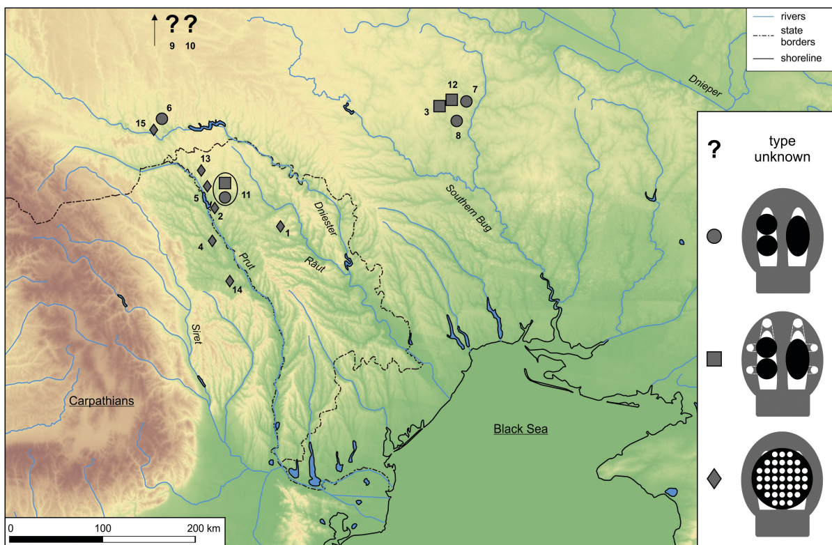
Fig. 14. Geographical distribution of the three techniques of managing the hot air inflow from combustion to firing chamber within the Cucuteni-Tripolye dual-chambered updraught pottery kilns in the IVth millennium BC. Numbers correspond to the ones from Table 2 (illustration S. Țerna)
