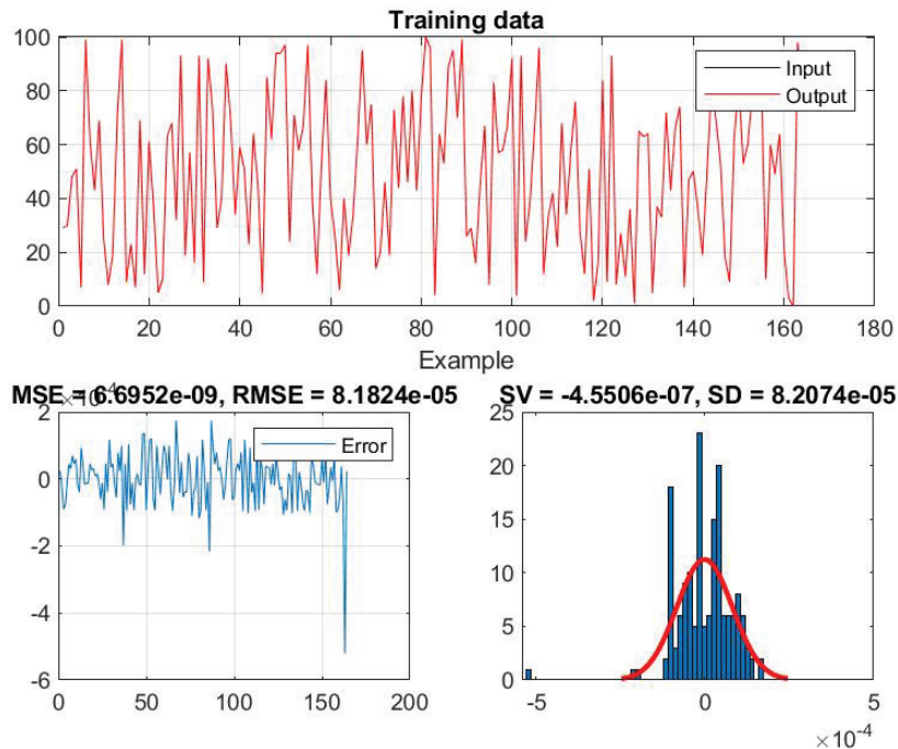
Figure 6. ANFIS network training - two inputs - achievements
